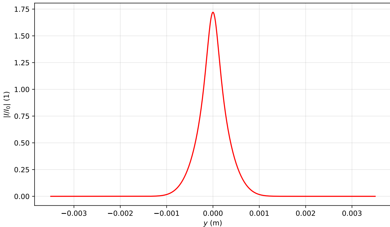
Intensity profile I(x = 0, y, z = 0.239)/I_0 , P_{in}=7.0P_{cr} , artificial time
